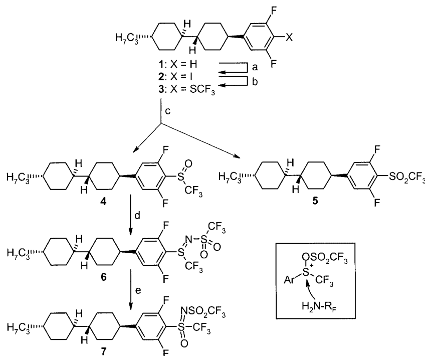
Scheme 1. Synthesis of the liquid crystals 3–7 : a) 1. BuLi, THF, -70 °C. 2. I 2 , THF, -40 °C (78%); b) CuSCF 3 , NMP, 120–150 °C, 18 h (56%); c) MCPBA, CH 2 Cl 2 , room temp., 3 d ( 4 : 28%; 5 : 7%); d) Tf 2 O, TfNH 2 , CH 2 Cl 2 , room temp., 18 h (16%); e) NaIO 4 , RuCl 3 (0.1 mol%), CH 3 CN, H 2 O, CCl 4 , room temp., 18 h (41%). The inset illustrates the reaction of the nucleophile (H 2 N-R F in this case triflic amide) with the sulfoxide activated by triflic anhydride.
